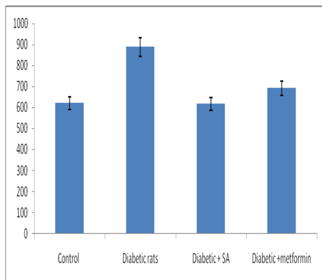
Fig.2. Effect of sinapic acid on the levels of glycogen phosphorylase in the experimental group of rats.
