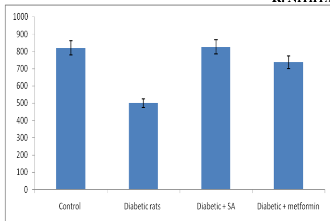
Fig.1. Effect of sinapic acid on the levels of glycogen synthase in the experimental group of rats.
