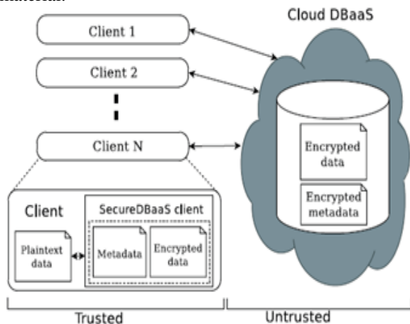
Fig.1. SecureDBaaS Architecture.
